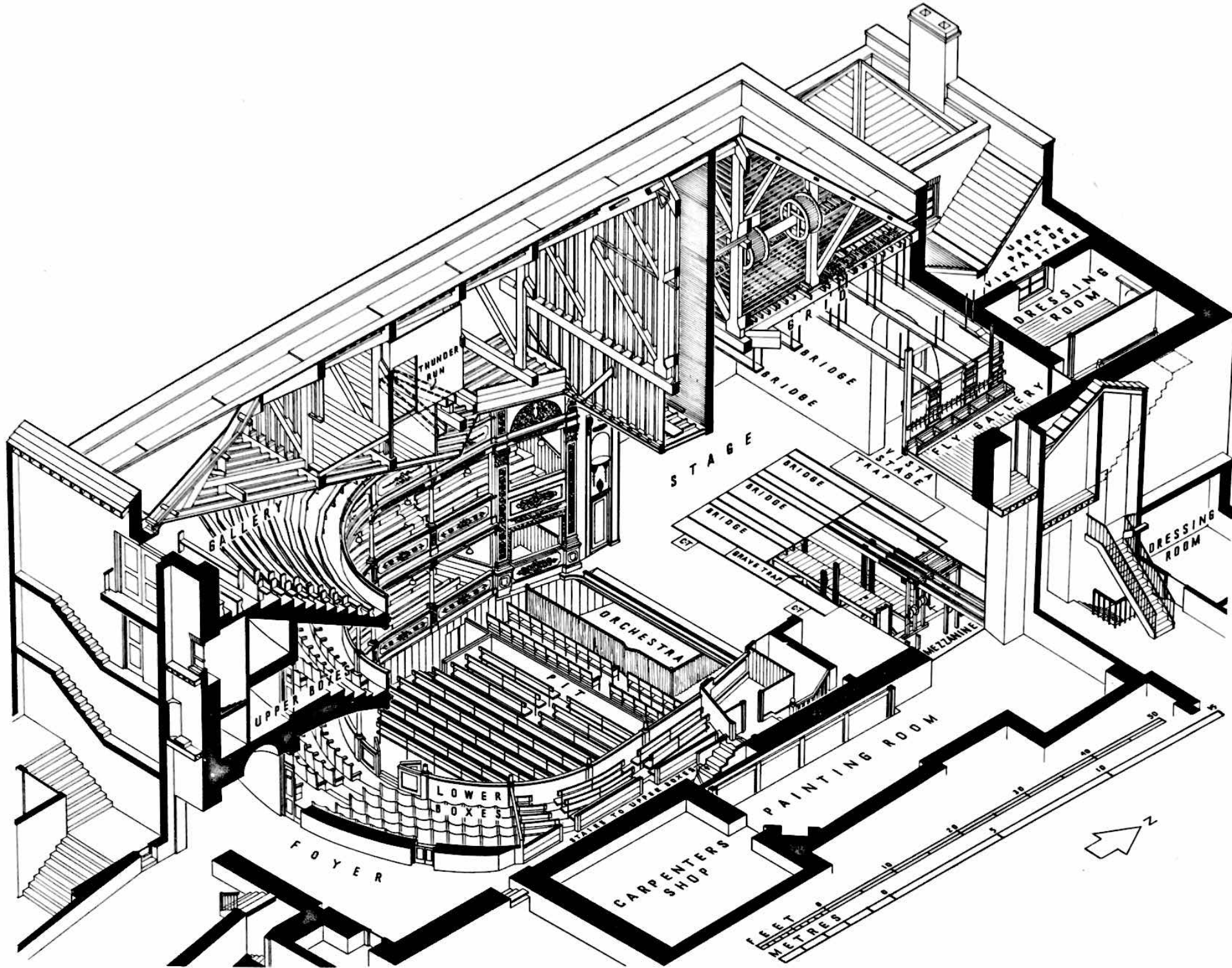
Fig.76. The Theatre Royal, Bristol, James Paty, 1764-6: scale reconstruction
