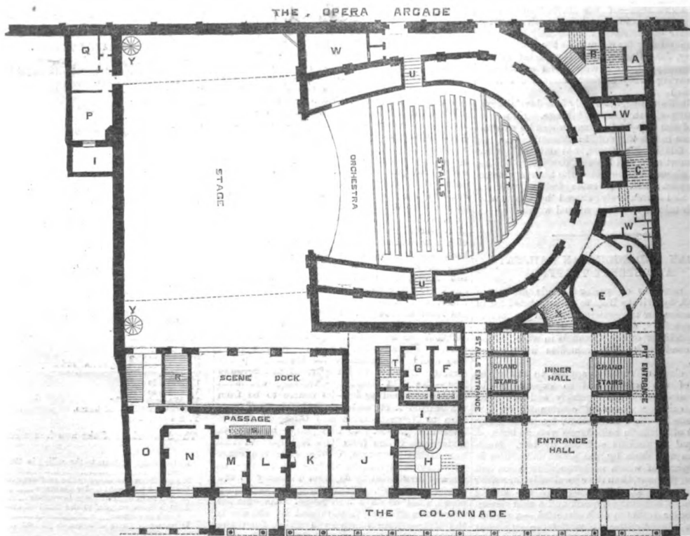
PLAN OF NEW THEATRE
