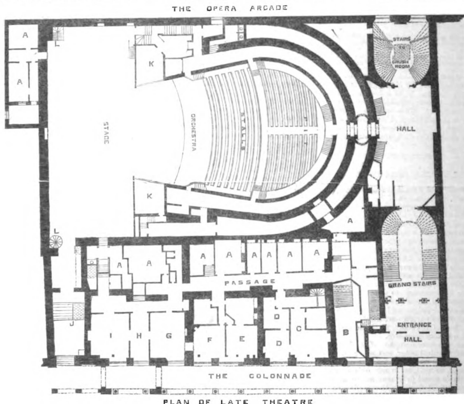
PLAN OF LATE THEATRE
