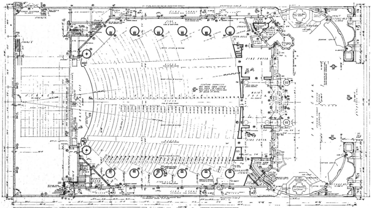
PLAN OF AUDITORIUM
